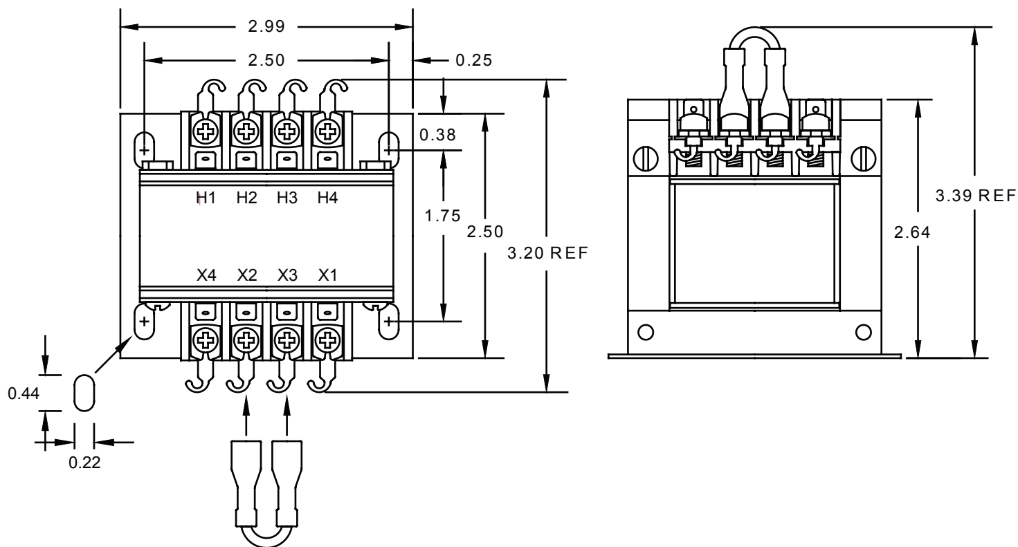
Figure 5. 480 Volt across H1 and H4 of Primary. Jumper across X2 and X3 to create 24 Vac on Secondary.
