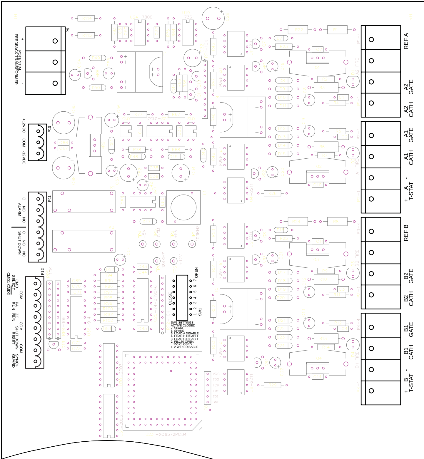
Figure 8. Remote Firing Circuit Board.
