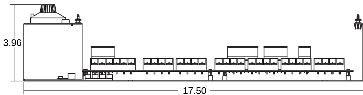
Figure 6. 3659 Remote Firing Circuit (Side view).
