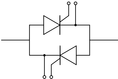
Figure 21. "AC Switch"
