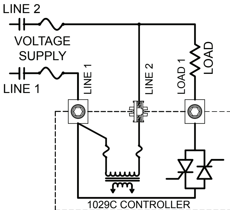
Figure 16. Power Path.
