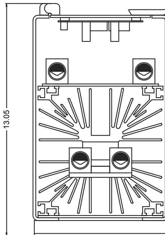
Figure 5. Installation drawing for 500 to 750 Amp units.
