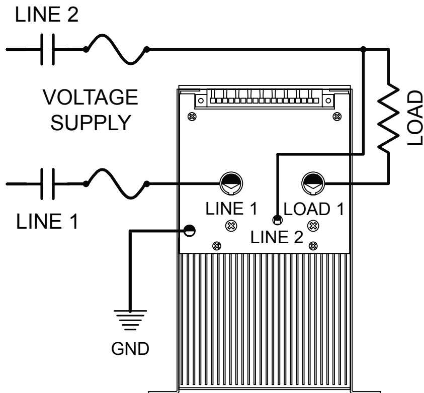
Figure 15. Power Connections.
