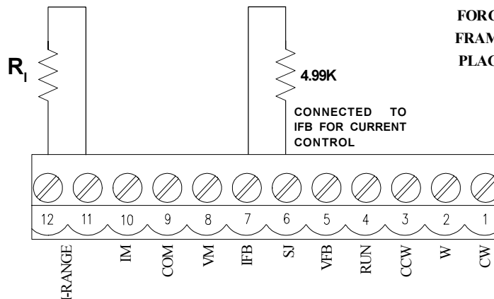
Figure 7. Current Feedback Resistor Connections.
