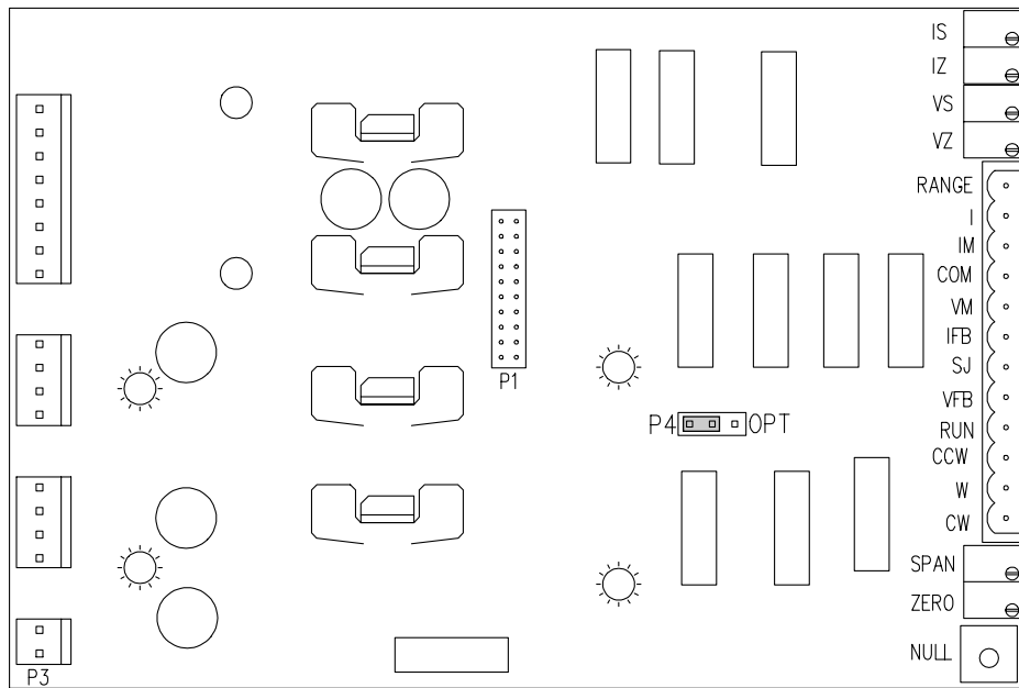
Fig. 9. 1039 board layout.
