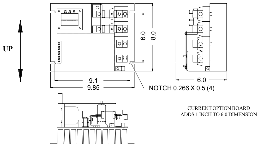
Fig. 13. Mounting dimensions of 55 to 75 amp frames.
