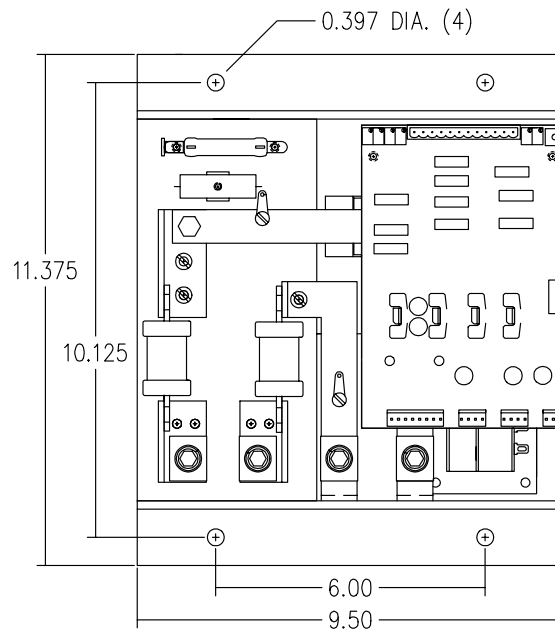
Fig. 14. Installation drawing of 90, 140 and 180 amp frame (top view).
